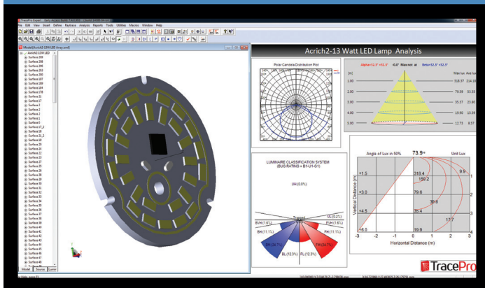
Acrich2-13W LED Array Report
