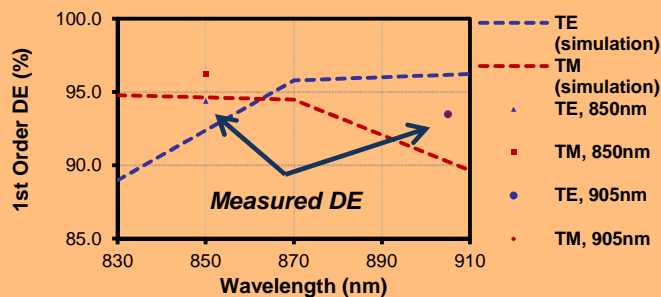
Diffraction Efficiency (Absolute): Holographix' Low-Scatter Transmission Grating (1200l/mm) Measured Values vs. Simulation
