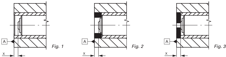
Fig. 1 Free space (without any stopper) for applications which doesn't require specific tolerances or exact ferrule axial positioning.
